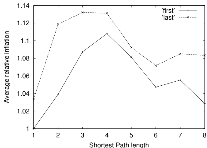
Fig. 16. Average relative inflation versus length of the topological path.
