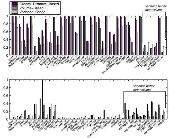
Figure 10: Affinity of heuristic algorithms to the optimal dynamic programming solution. Top : Closeness of absolute distances to optimal (numbers closer to 1 are better). Bottom : Closeness of relative distances to optimal (numbers closer to 0 are better).
