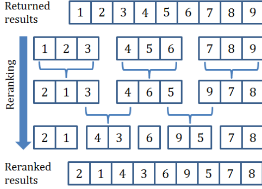
Fig. 4. Illustration of the reranking process. In this case, the returned results are first split into non-overlapping windows, each containing 3 subjects. Reranking is performed using SB distances, subjects with the lower SB distances are moved to front. Adjacent matches from different windows are then reranked to output smooth results.
