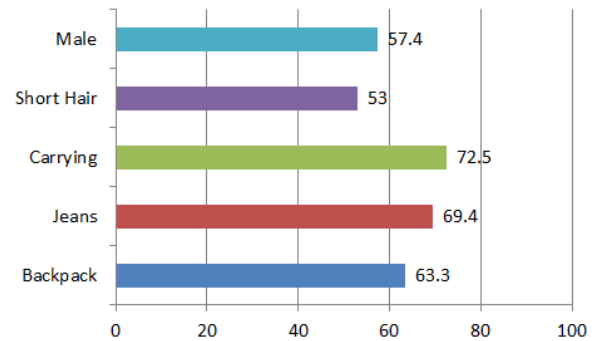
Fig. 5. Attribute detection accuracy for the 5 SB attributes used in this paper (in %).
