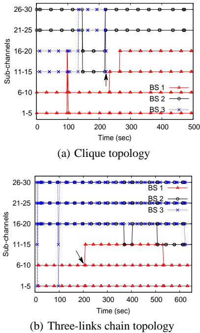
Figure 11: Convergence of RADION with network dynamics.
