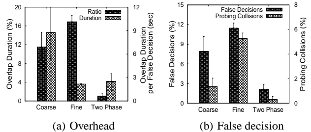
Figure 8: Two-phase adaptation outperforms other schemes.
