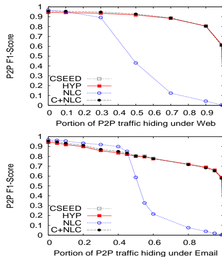
Figure 9: Obfuscation by blending for the BRAZ trace. P2P traffic is trying to tunnel its traffic using on of the following two applications: WEB (top plot) and EMAIL (bottom plot).
