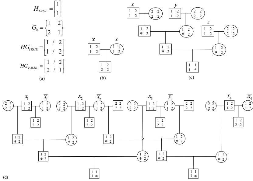
Fig. 4. (a) G_0 , H_{TRUE} , HG_{TRUE} and HG_{FALSE} . (b) Gadget for variable x . (c) Gadget for clause z . (d) An example of the reduction from 3SAT to 2-locus-MRHC* for (x_1 \vee x_2 \vee x_3) \wedge (\bar{x}_2 \vee \bar{x}_3 \vee x_4) .
