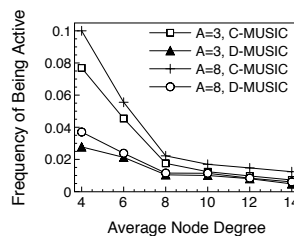
Fig. 4. The frequency with which sub-topologies are activated with C-MUSIC and D-MUSIC
