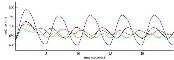
Figure 6: Volume for various breath styles. The shown tidal (peak-to-peak) volumes computed for our simulation's lung cavity fall within the realistic human range, with the calm breath (shown in black) falling almost perfectly on the 500 mL average quoted in the texts. Computed post-mortem, this reveals a strong correspondence between our results and that of real human motion.
